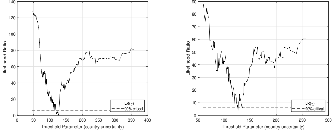
Figure 1: Confidence interval construction for threshold
