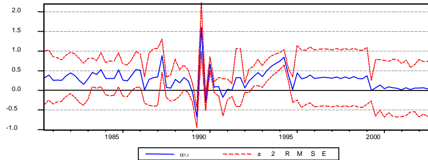
Graph 4 – IGP-DI: Smoothed Estimate of \alpha_{1,t}
