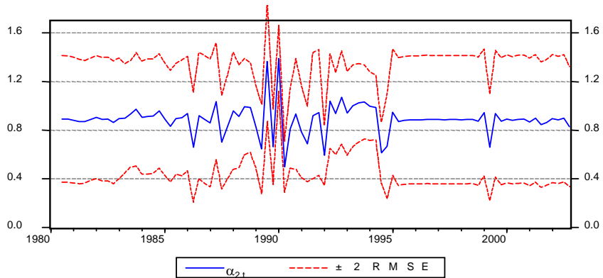
Graph 6 – IPA: Smoothed estimate of \alpha_{2,t}
