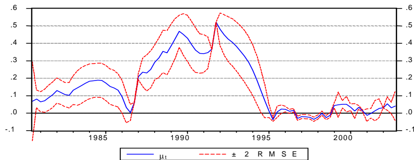
Graph 1 – IPCA: Smoothed Estimate of \mu_t
