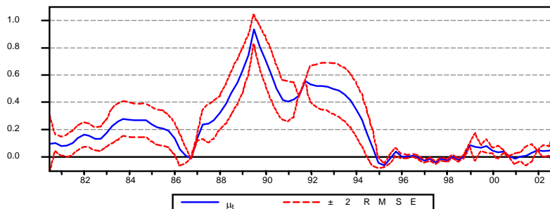
Graph 3 – IGP-DI: Smoothed Estimate of \mu_t
